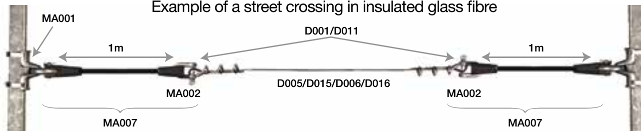
Example of a street crossing in insulated glass fibre
